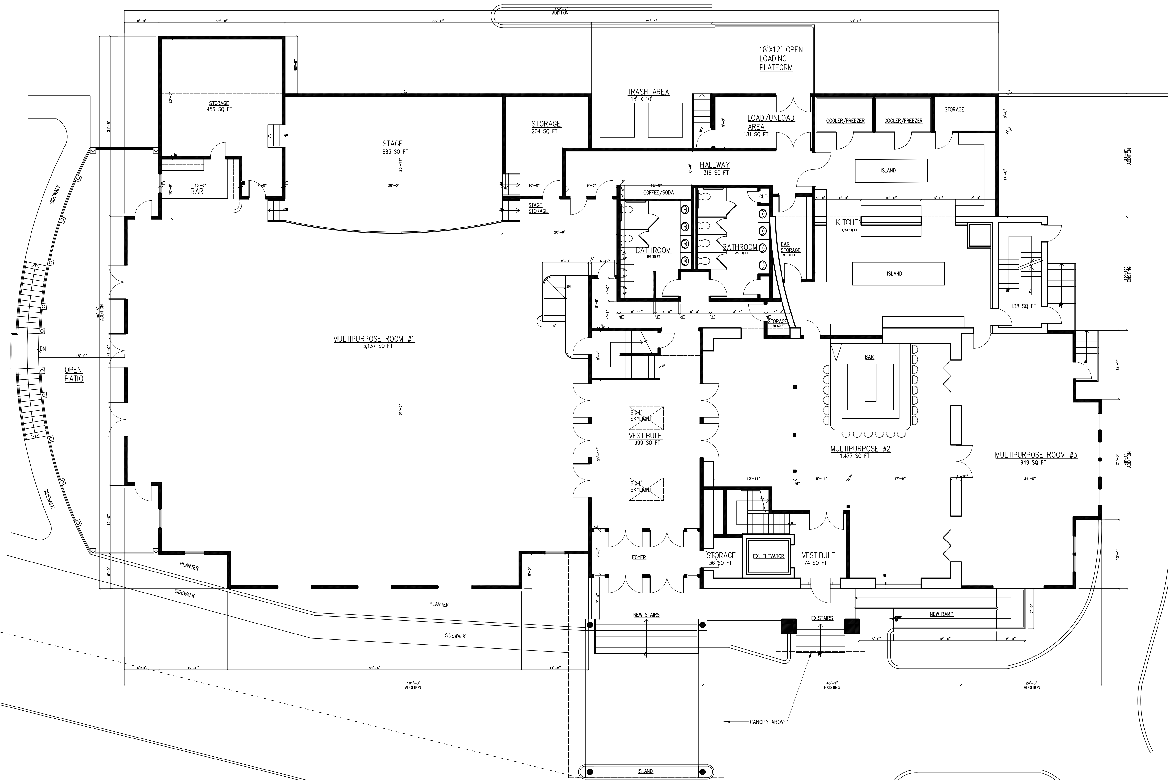
FIRST FLOOR PLAN SCALE: 1/8" = 1'-0" 13,689 SQ FT TOTAL
