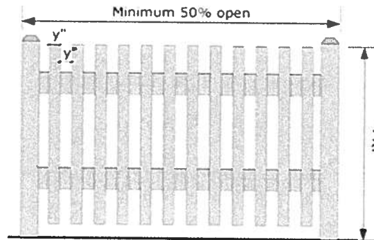
Figure 17.6.6: Fifty-percent Open Fence
